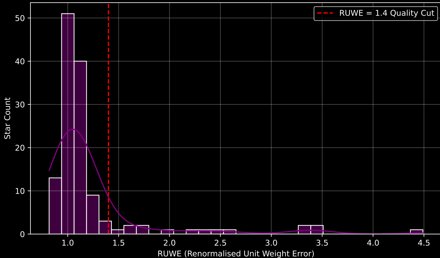
GALAH DR4 Field [6586] RUWE Distribution (n= 131)
