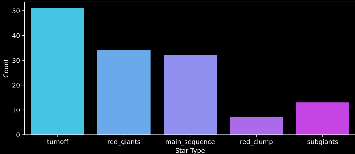
GALAH DR4 Field: [6586] Count plot of Star Type
