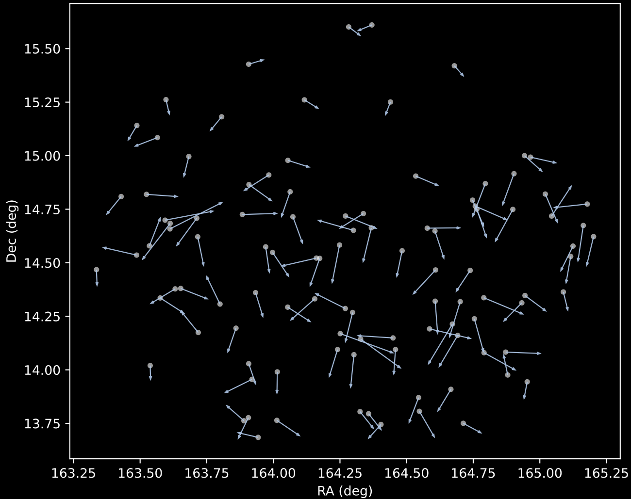
GALAH DR4 Cluster 1 Proper Motion Vectors (n=103)
