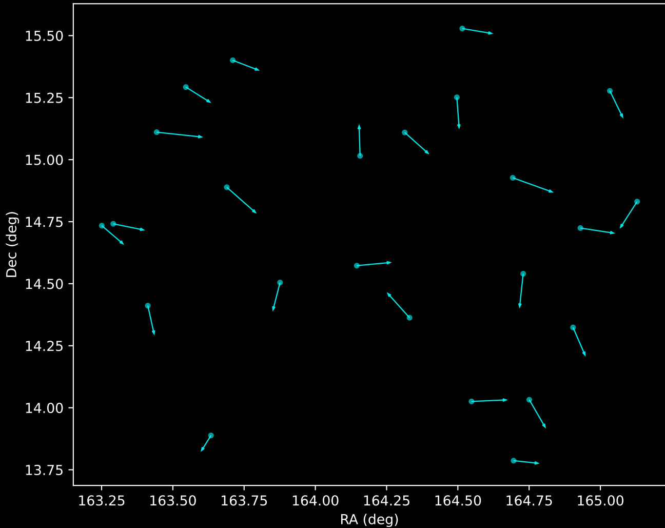
GALAH DR4 Noise Stream Proper Motion Vectors (n=24)
